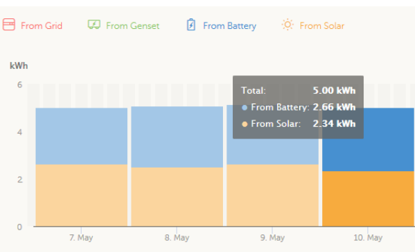
Solar AQMS daily consumption distribution
